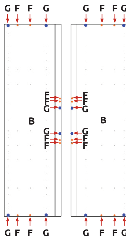
DOWEL (F) & CAM DOWEL (G) LOCATION DETAIL
